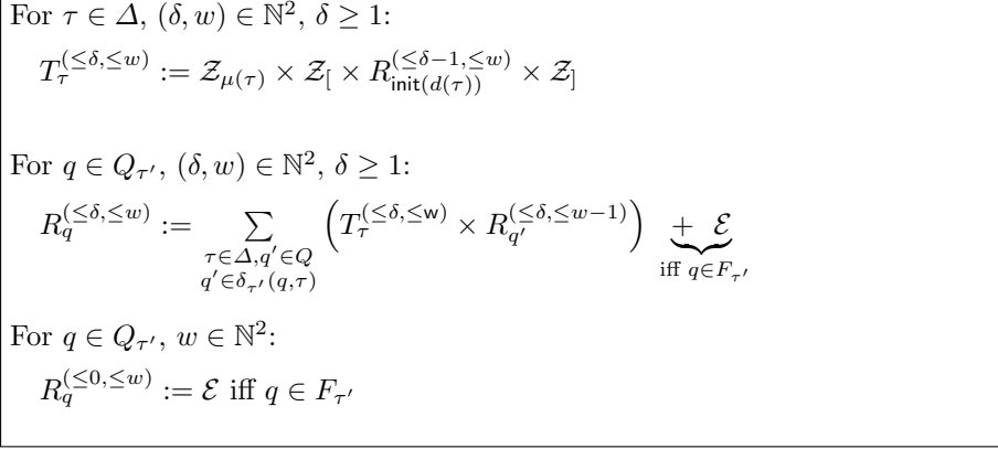
Fig. 4.1 Combinatorial specification of CFG G_D in the presence of shape constraints.
