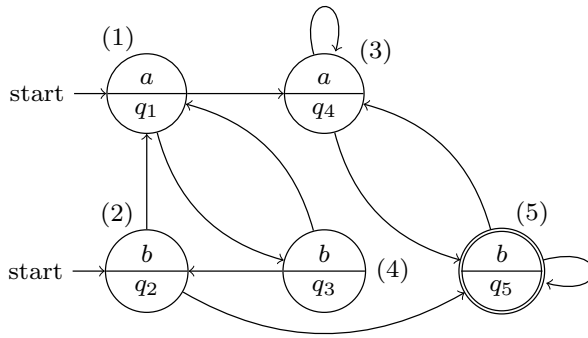
Fig. 6.1 An example of an admissible k -occurrence automaton ( k -OA).
