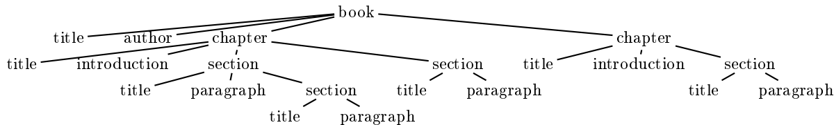
Figure 3: A document conforming to the schema of Example 3.
