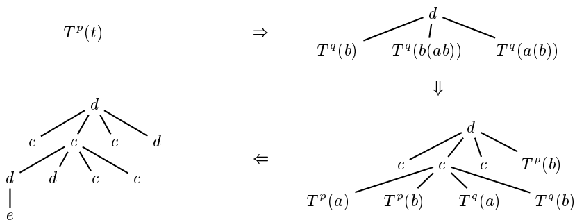
Figure 2: The translation of t = b(bb(ab)a(b)) by the transducer T of Example 1.
